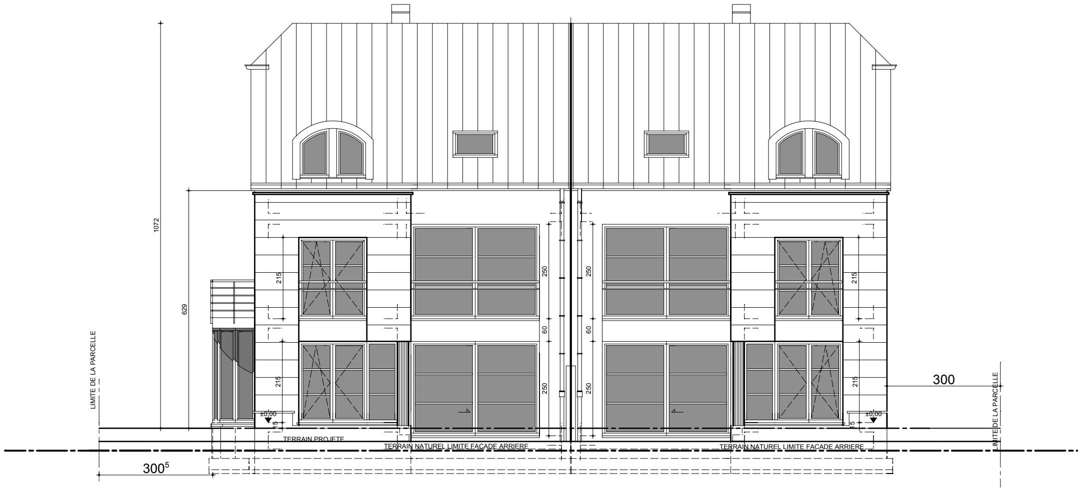
FACADE ARRIERE
